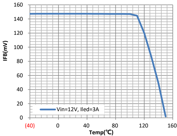
Temperature vs. I FB
